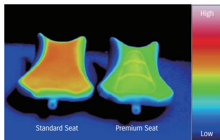
Thermographic comparison of surface temperatures
